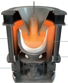
Furnace insulation
